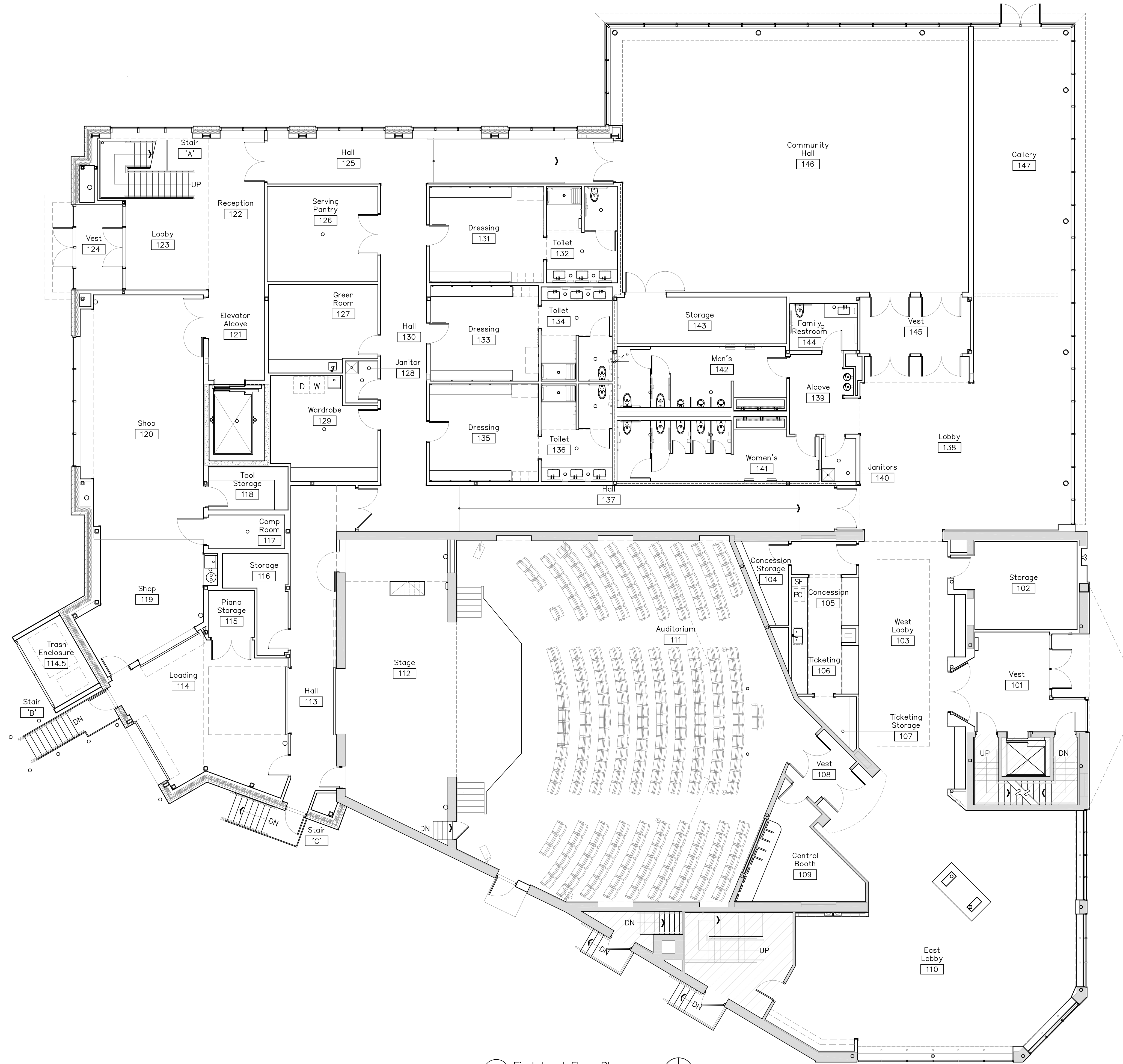
A3 First Level Floor Plan 1/8"=1'-0" NORTH
